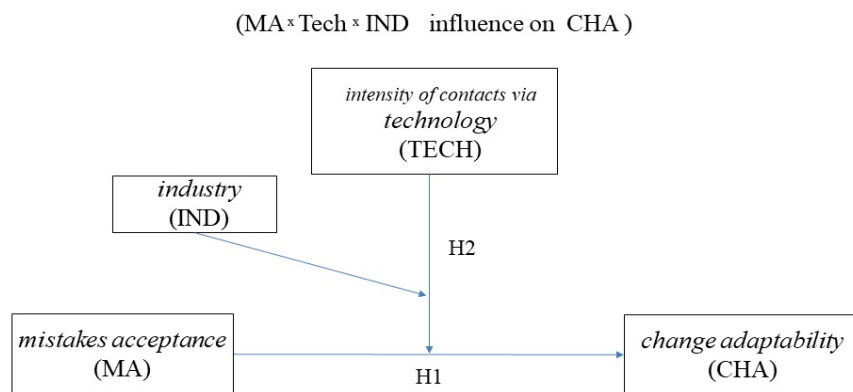
Figure 1: Theoretical model
